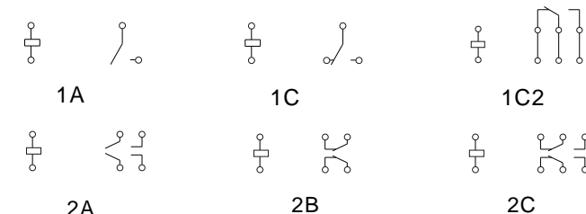
Wiring diagram (Bottom view)
