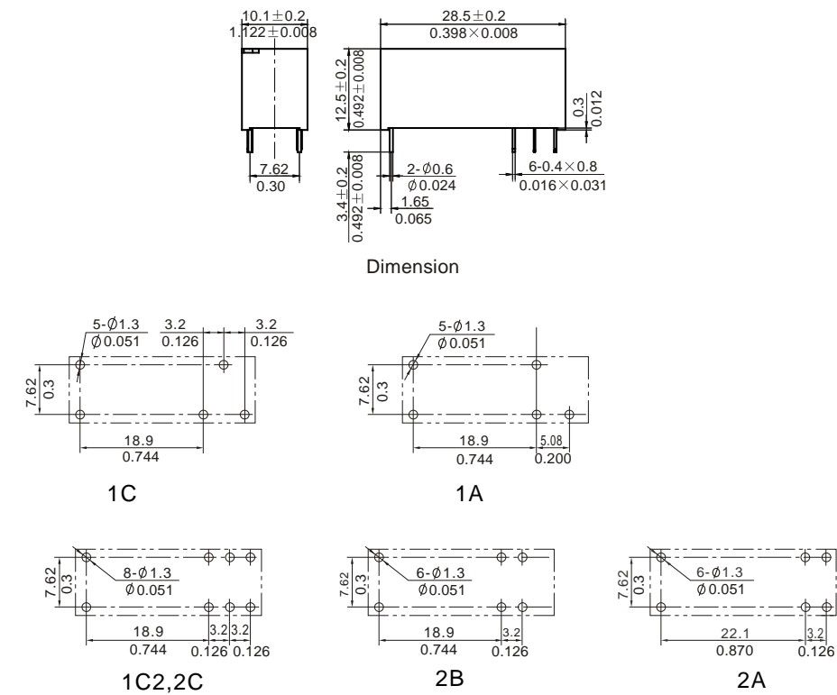
Mounting (Bottom view)
